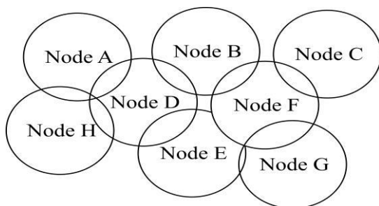
Figure 2: Ad-hoc Network
